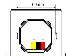
Figure 7. Dimensions - Back View (EU)
