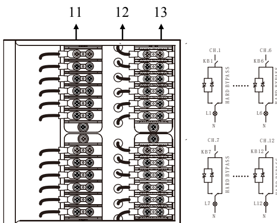
Jumper wiring terminal
