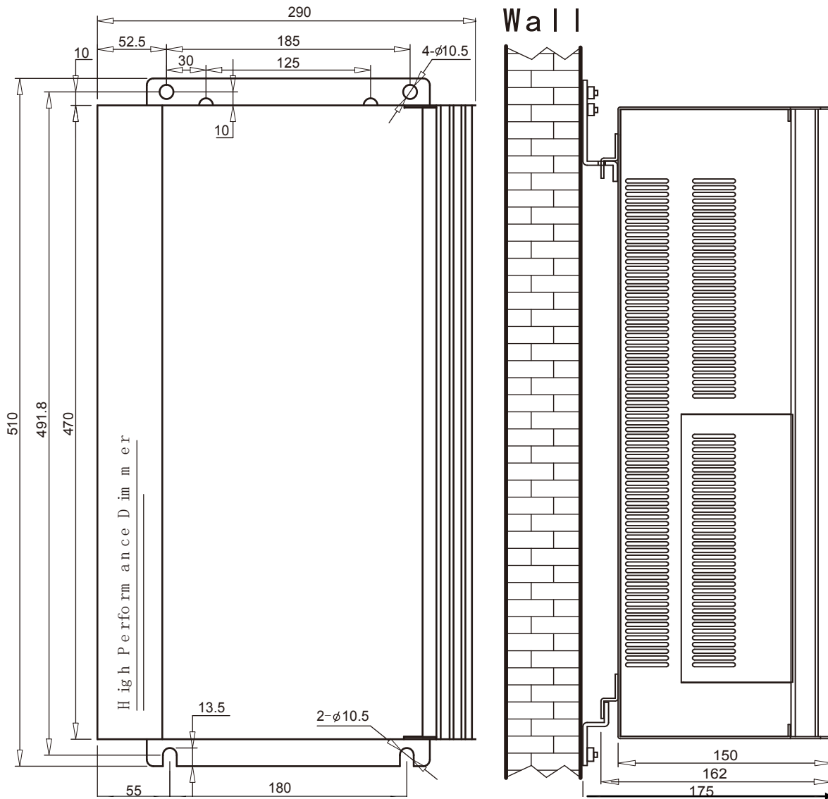
Installation dimensions
