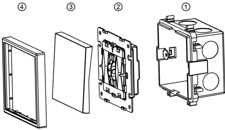
Figure 4. Installation
